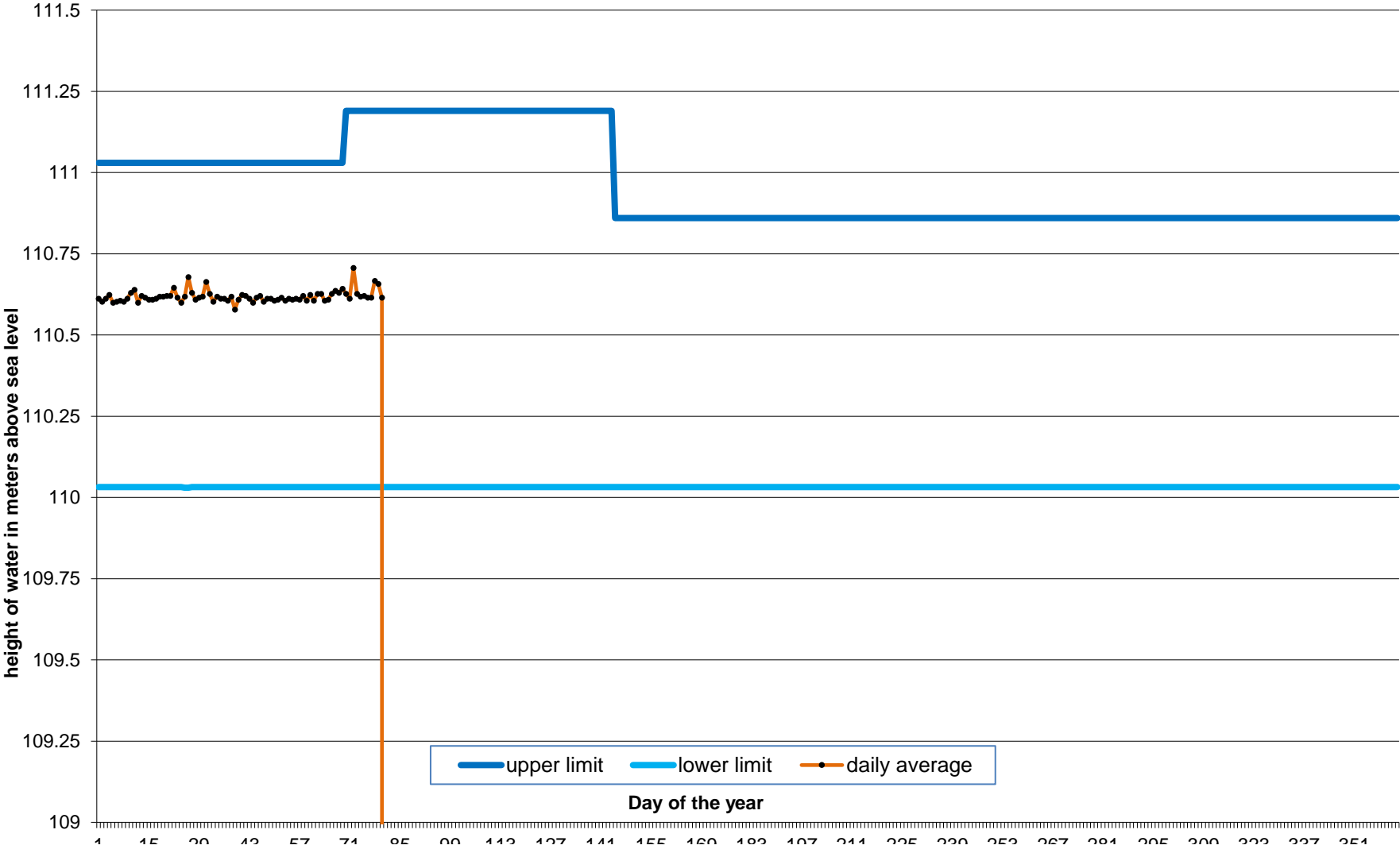
RPG 2020 Levels for Dam #1 Jan 1 to Mar 22
