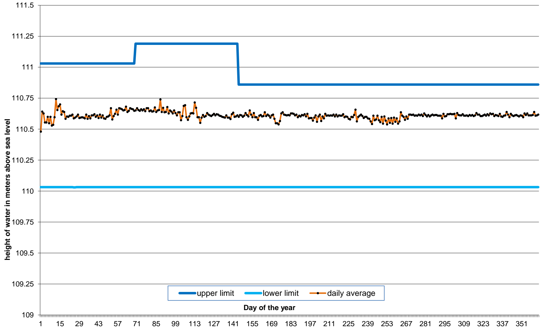
RPG 2018 Levels for Dam #1 Jan 1 to Dec 31
